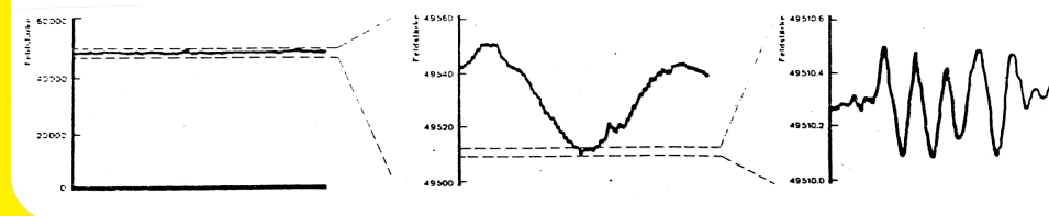
Fig. 22: Variations in earth's magnetic field: Sensitivity of the measurements increased a 1000 times in each case. Diurnal rhythms and micro-pulsations are visible, utilised by bees and other organisms for orientation in space and time.
