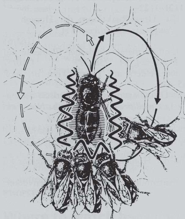
Fig. 21: The waggle dance of the bees generates electrical oscillating fields. Warnke 1989, Copyright Ulrich Warnke
