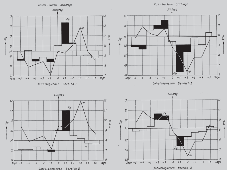
Fig. 6: Significant synchronicity of very long waves and contracting poliomyelitis. The black bars show days of low (bars downward) or high (bars upward) sferics activity and the superimposed curves show the correlated levels of poliomyelitis contraction in the fifties.
