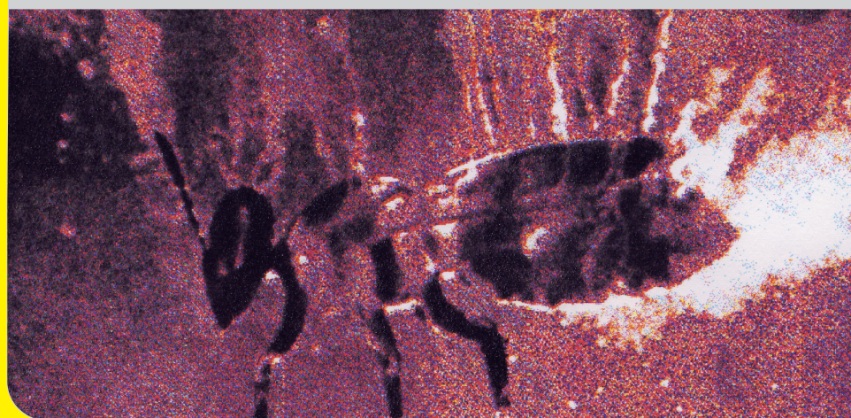
Fig. 11: A bee in an electrical field; top: a construction, bottom: an experiment. It is shown how the field strength increases around certain surface structures.
