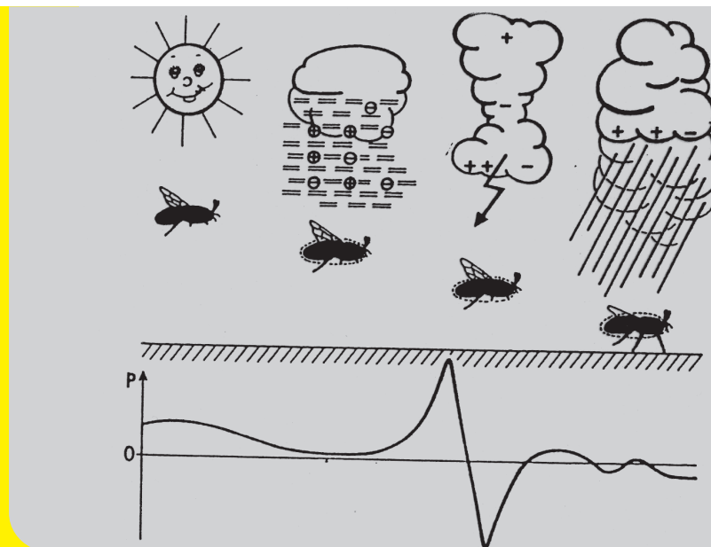
Fig. 2: Top sketch: The electrical charging of the insects changes typically as the weather parameters change. The bottom curve shows the changes in the electrical field of a freely flying bee as a function of the weather condition.
